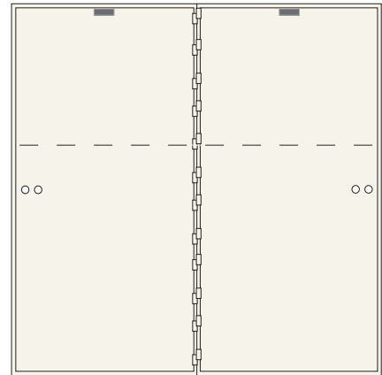
AXL-2-33 (Wt. 280 lbs.) 2 openings ea. 33" x 16"
