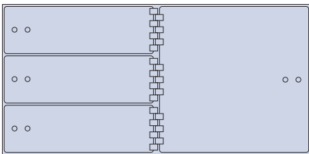
TLX-4R (Wt. 180 lbs.) 3 openings ea. 4 1/2" x 15" and 1 opening ea. 15" x 15"
