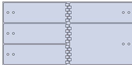
TLX-5R (Wt. 180 lbs.) 4 openings ea. 4 1/2" x 15" and 1 opening ea. 10" x 15"
